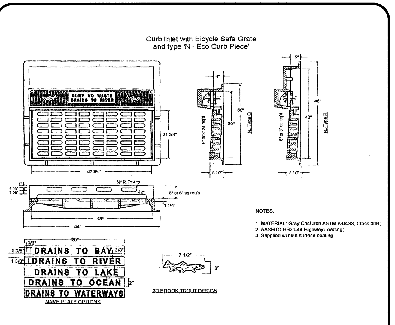
HEAVY DUTY BICYCLE SAFE GRATE N.T.S.
