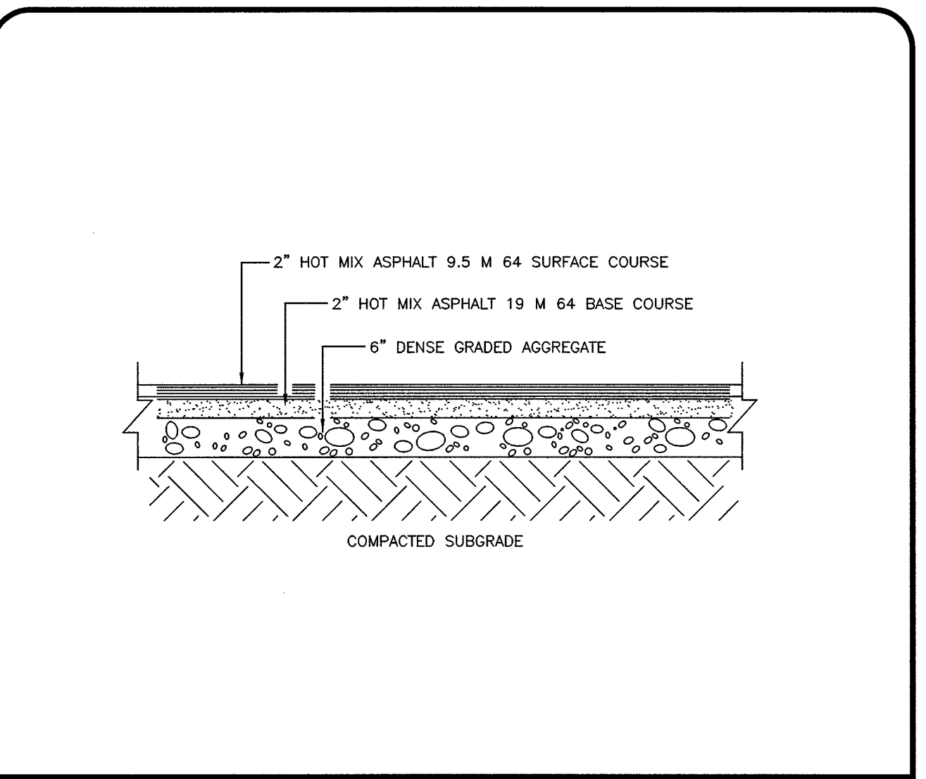
ASPHALT PAVEMENT DETAIL N.T.S.
