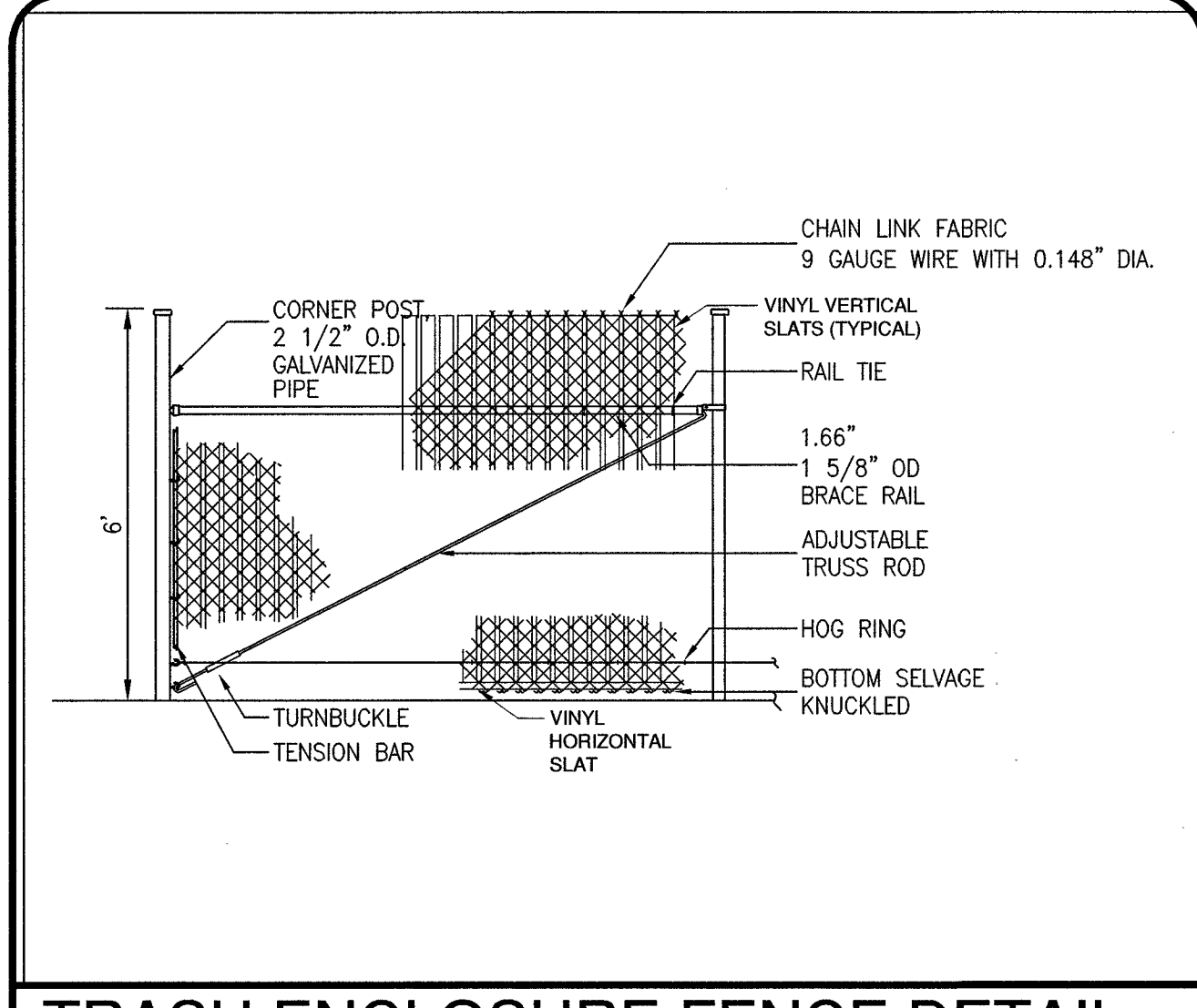
TRASH ENCLOSURE FENCE DETAIL N.T.S.
