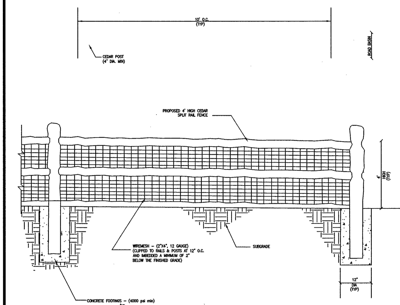
SPLIT RAIL BASIN FENCE DETAIL
