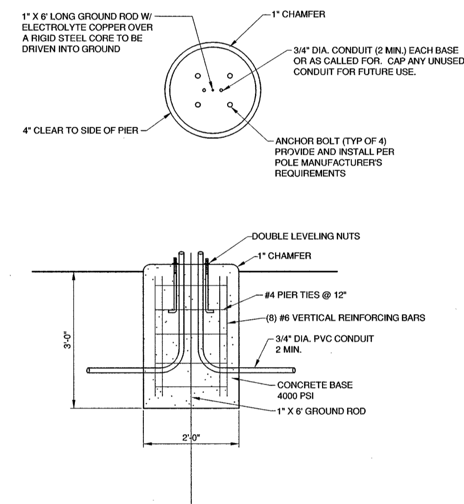
LIGHT POLE BASE DETAIL
