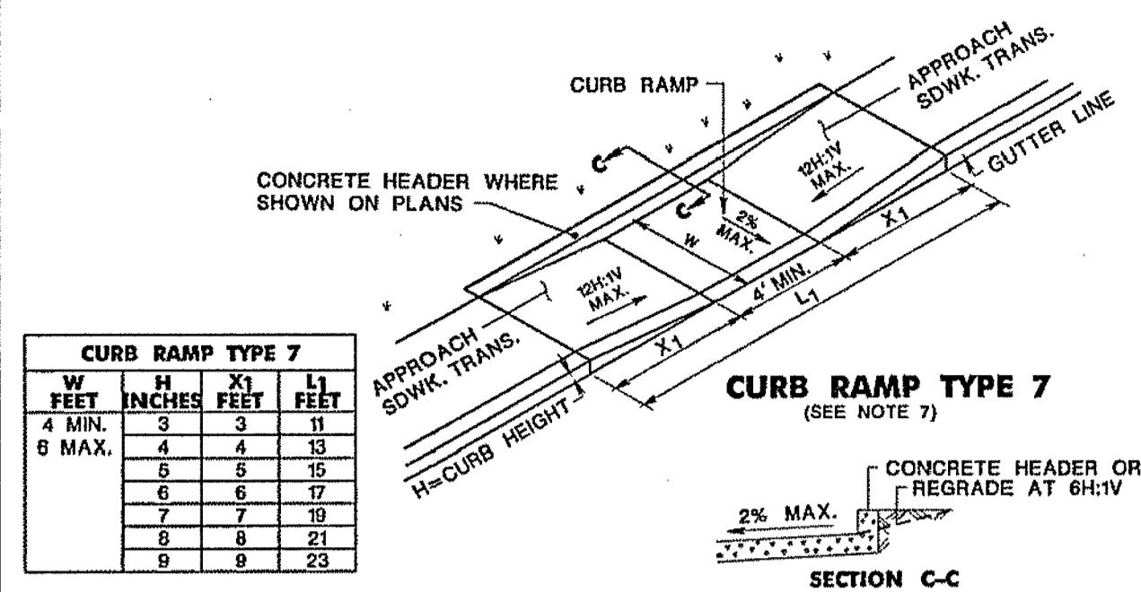
NJ DOT TYPE 7 HANDICAP RAMP DETAIL
