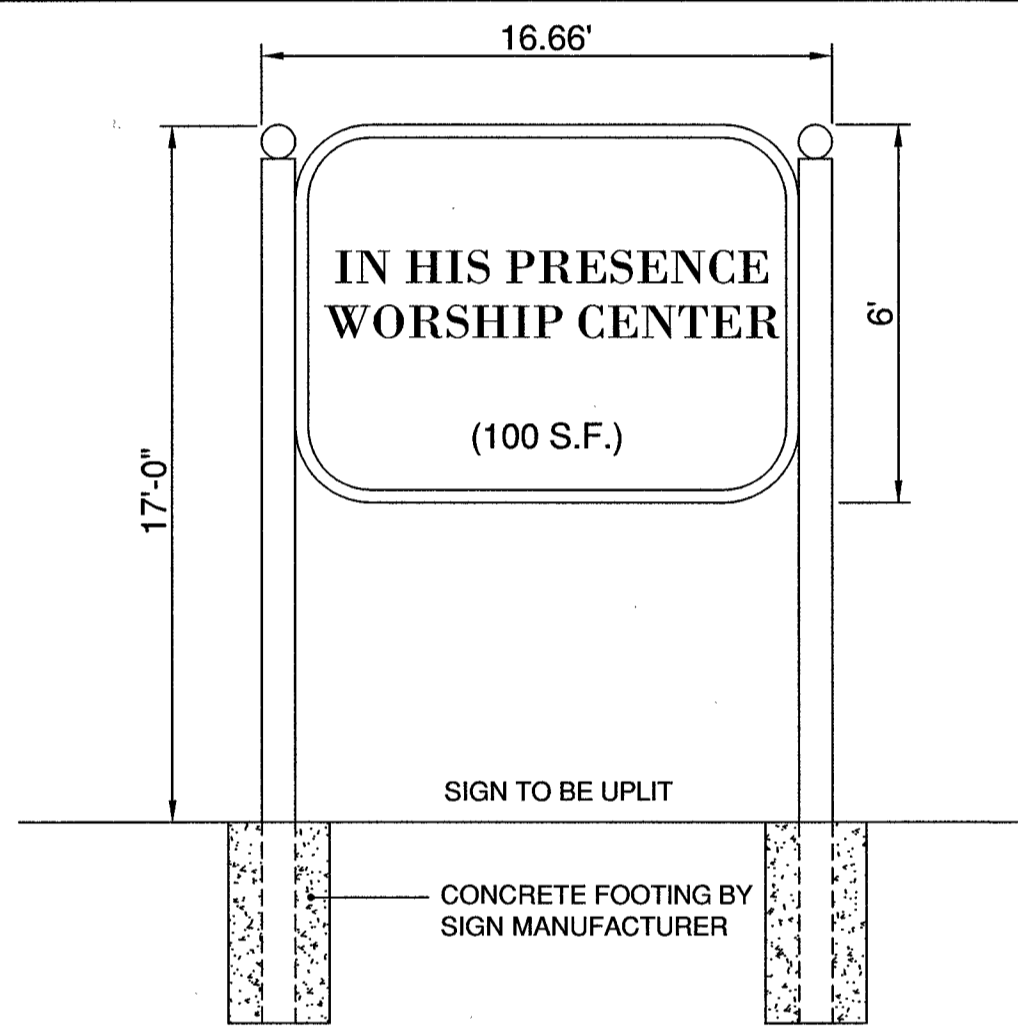
FREESTANDING SIGN DETAIL
