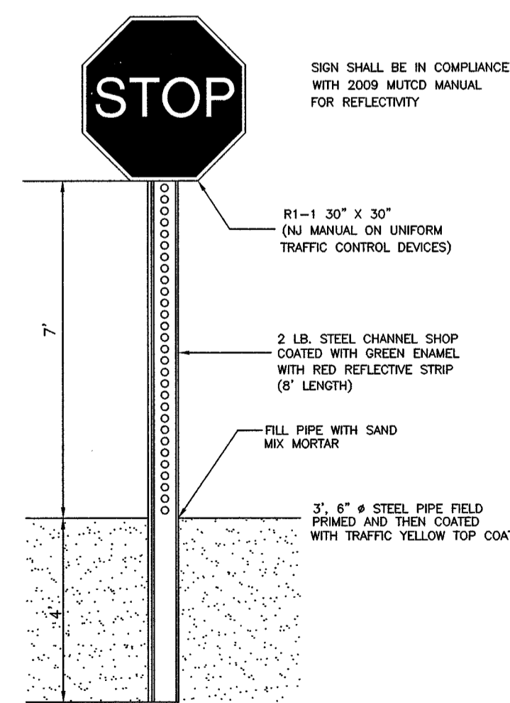
STOP SIGN DETAIL
