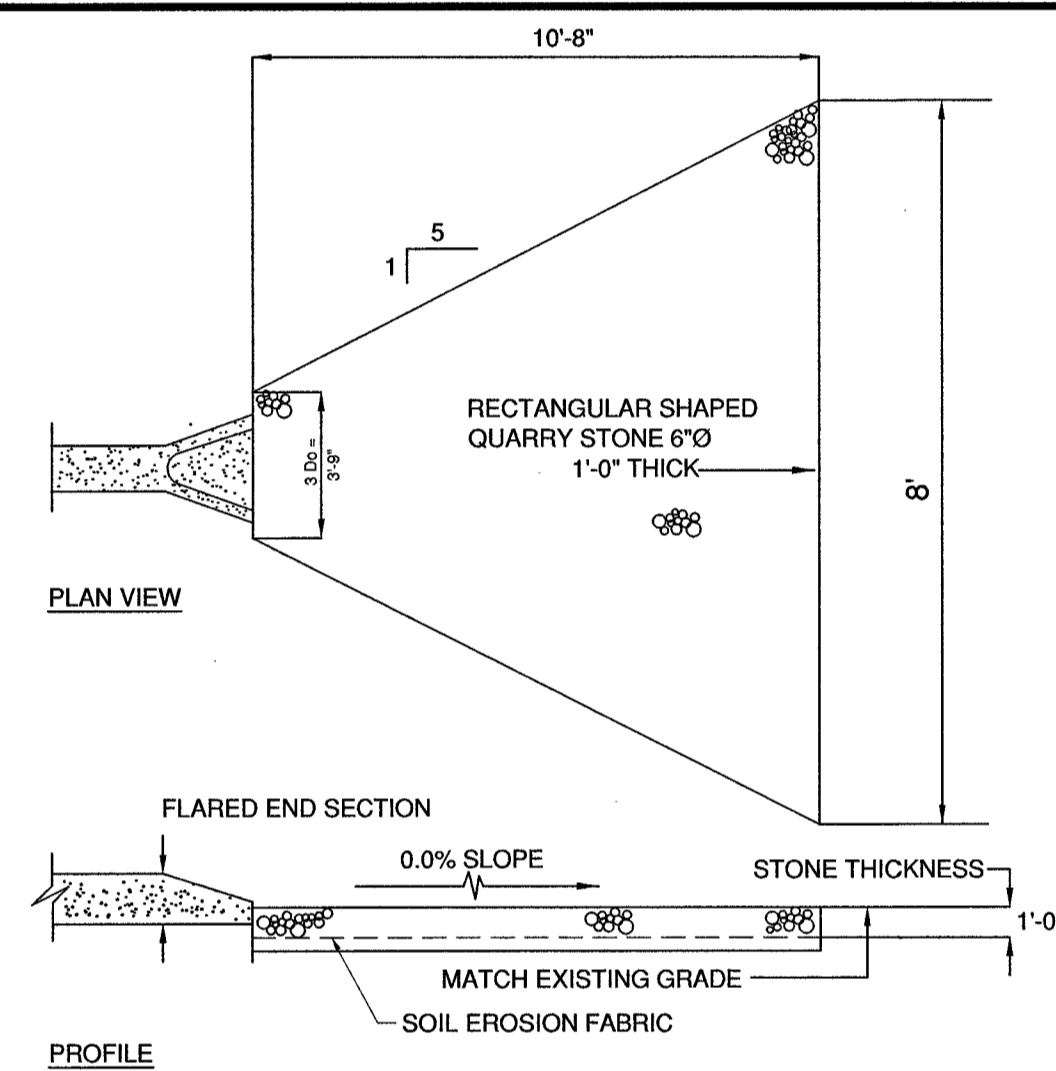
STONE APRON DETAIL #1
