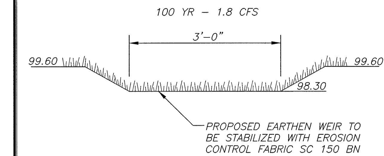
EMERGENCY WEIR DETAIL
